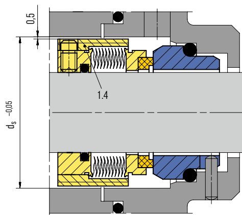
MFL85F
