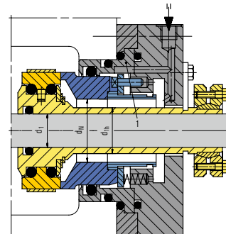
HR3
