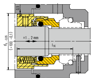
H7F/H75®F
