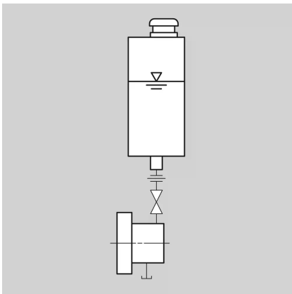
P&ID for QFT6 quench system according to API 682 4th edition.
