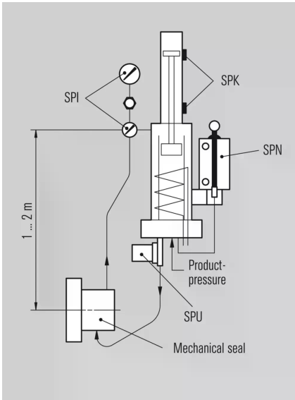
Operating and installation diagram for a DRU system.
